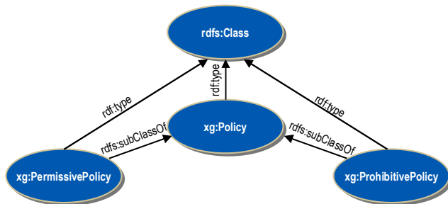
Figure 3. XG Policy Language model.
